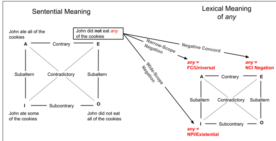
Figure 1: Two Aristotelean squares of opposition illustrate three possible mappings from sentential meaning (left) to the lexical meaning of any (right). If a sentence containing any under a negator is correctly understood to have a universal negative meaning (the E corner of the left square), there are three consistent analyses of the lexical meaning of any (three arrows). If the sentence is analyzed as a negative concord construction, the lexical meaning of any would be analyzed as a negator (the E corner of the right square). If the sentence is analyzed with inverse scope ( any taking wide scope over not ), any would be a universal quantifier or free-choice operator (the A corner of the right square). If the sentence is analyzed with linear scope ( not taking wide scope over any ), any would be an existential quantifier (the I corner of the right square). Note that two of these analyses yield contradictory lexical meanings (I and E).
